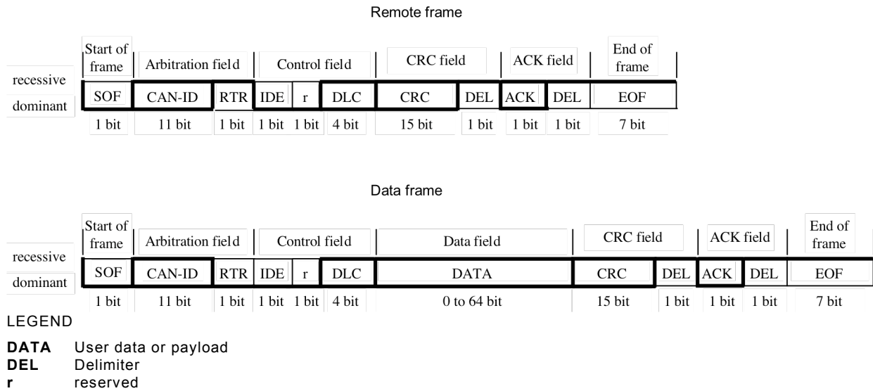
Figure 1 – Format of the CAN data and remote frame with 11-bit CAN-ID
