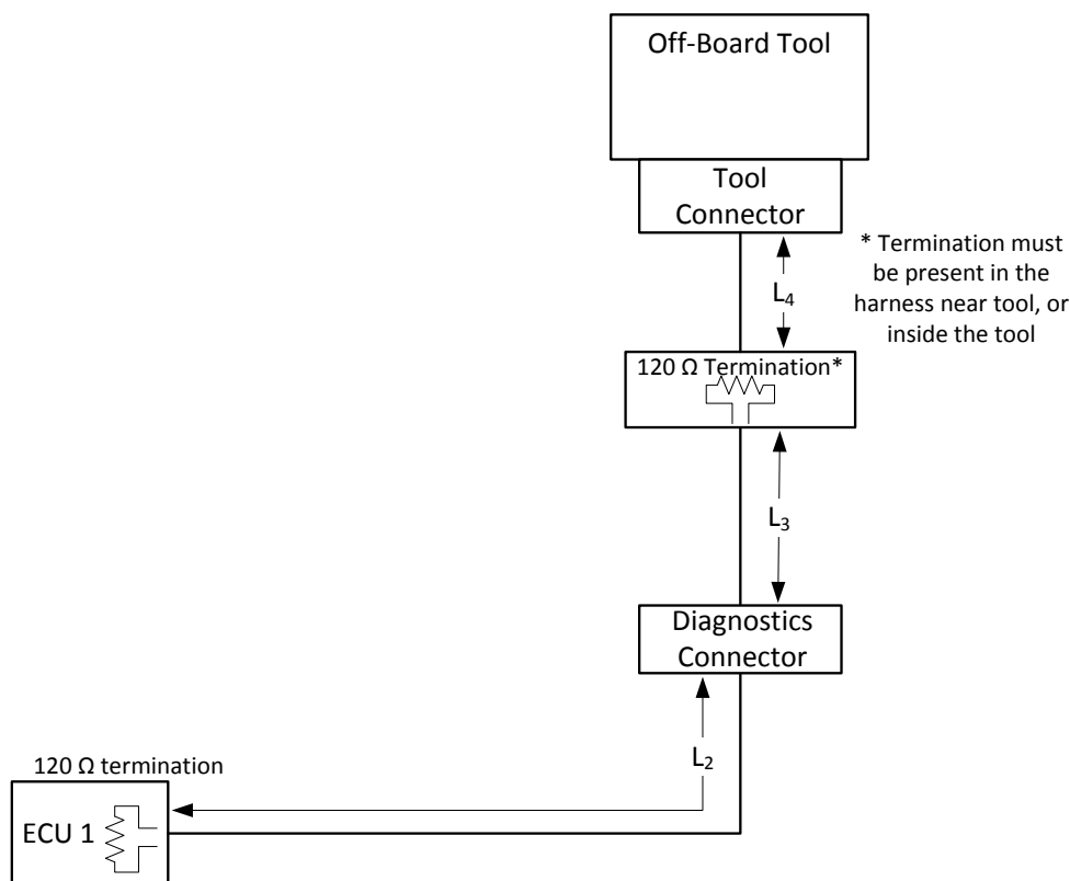
Figure 1 – Single on-board ECU configuration A
