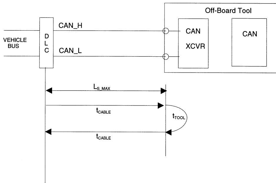
Figure 3 - Off-board tool parameters
