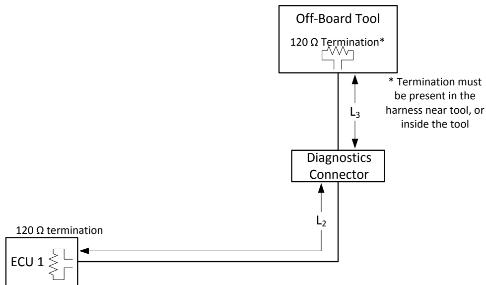
Figure 2 – Single on-board ECU configuration B
